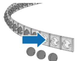
Press rolling elements into cage
